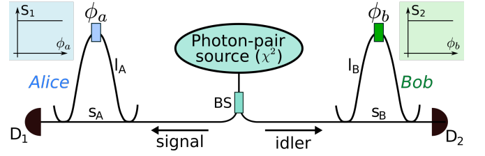
FIG. 8. Principle for generating and analysing energy-time entangled photons, as explained in Ref. [27]. A source generates a flux of energy and time correlated photon pairs, which are sent, after separation at a beam-splitter (BS), to two unbalanced interferometers at Alice's and Bob's sites (Franson configuration [109]). The individual photons can either travel along a short or a long path ( s_{A,B} or l_{A,B} ). The phase difference between the two arms is given by \phi_{A,B} , and the path length difference in both interferometers is set to be bigger than the coherence time of the individual photons to avoid single photon interference at each interferometer's output. In half of the cases, both photons take opposite paths. In the other half of the cases, both photons take the same path ( s_A - s_B and l_A - l_B ), and those events can be post-selected from the others by time-tagging. If both photons exit the interferometer through the bottom output (towards detectors D_1 and D_2 ), then they are projected into the following state: |\psi\rangle \propto |s_A\rangle|s_B\rangle + e^{i(\phi_A + \phi_B)}|l_A\rangle|l_B\rangle . The contributions |s_A\rangle|s_B\rangle and |l_A\rangle|l_B\rangle become indistinguishable when the photon pair generation time is unknown to more than the travel time difference between short and long paths, which can be achieved by a continuous wave pump laser for which the spontaneous generation of photon pairs inside the PPLN/W occurs at totally random times (energy-time entanglement). Or, a pulsed pump may be used, for which photon pairs can be spontaneously generated at two different times, which match the travel time difference of the interferometers (time-bin entanglement). Both strategies make it impossible to know whether both photons took the short or long paths. In this case, entanglement is observed, which is expressed as a phase-dependent sinusoidal oscillation of the two-photon coincidence rate, R_c , between the two detectors, R_c \propto 1 + V \cdot \sin(\phi_A + \phi_B) . Here, V is the visibility of the interference fringes, which has to be above 71% to demonstrate the presence of entanglement.
